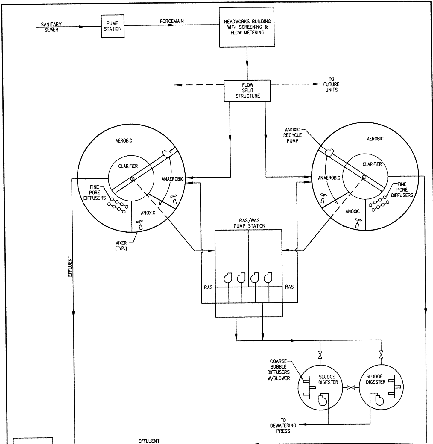
FIGURE 7-11 TREATMENT OPTION 3 BNR PROCESS PROCESS FLOW SCHEMATIC
