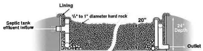
Figure 7. Rock-plant filter.
