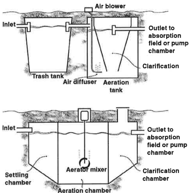
Figure 6. Aeration systems.
