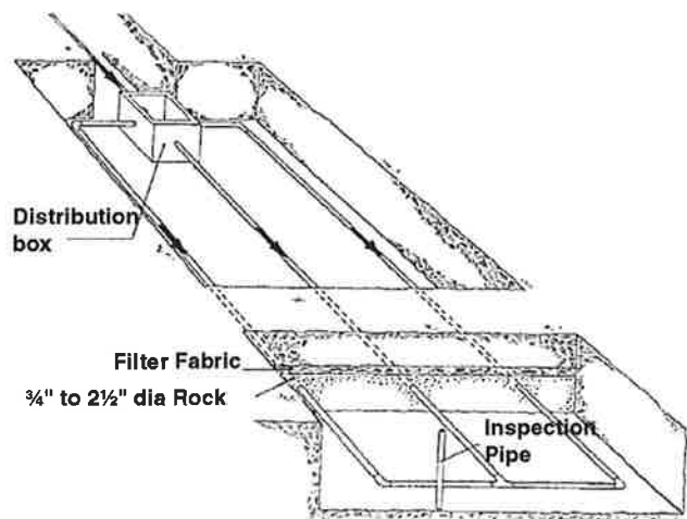
Figure 9. Absorption Bed.
