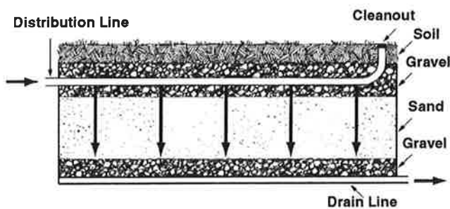
Figure 4. Sand filter.
