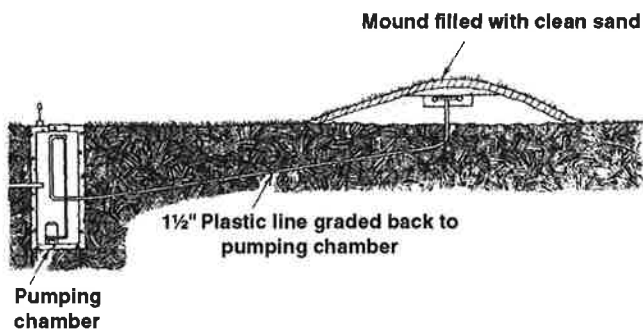
Figure 5. Mound.
