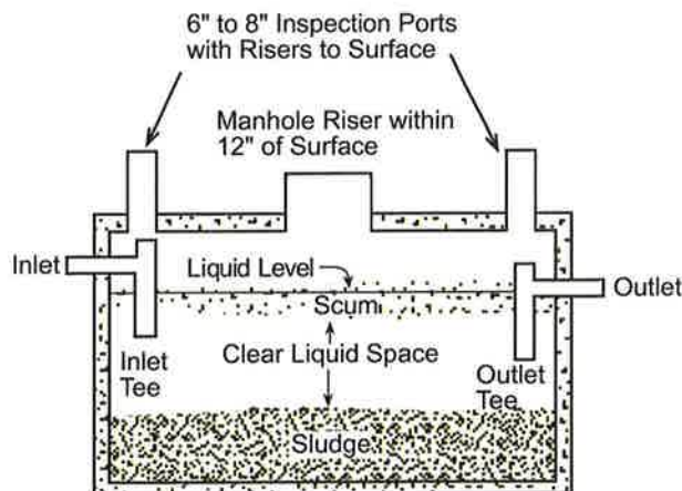
Figure 1. Cross Section of a Septic Tank
