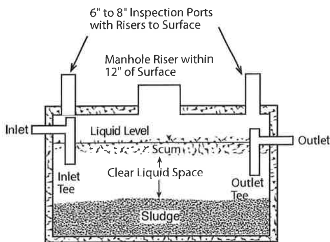
Figure 1. A septic tank designed for easy maintenance.
