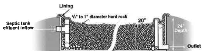
Figure 7. Rock-plant filter.
